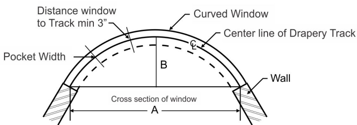
FIGURE 3: CRITICAL DIMENSIONS OF A CURVED TRACK
