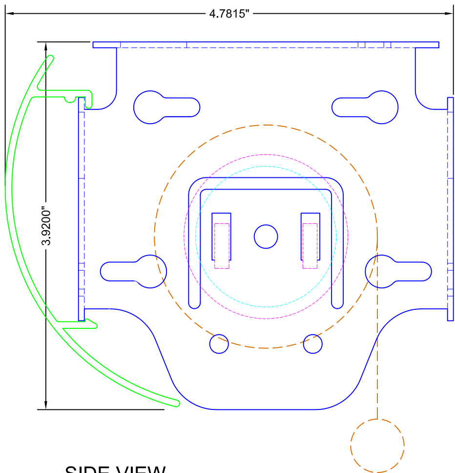
SIDE VIEW
